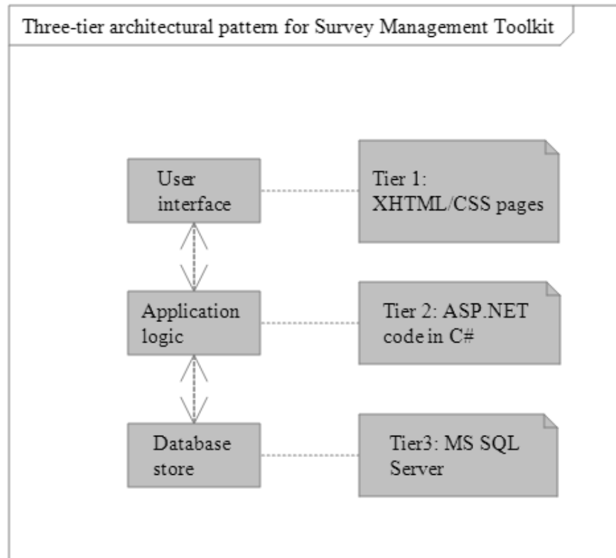
Figure 5.3: Three-tier architectural pattern
