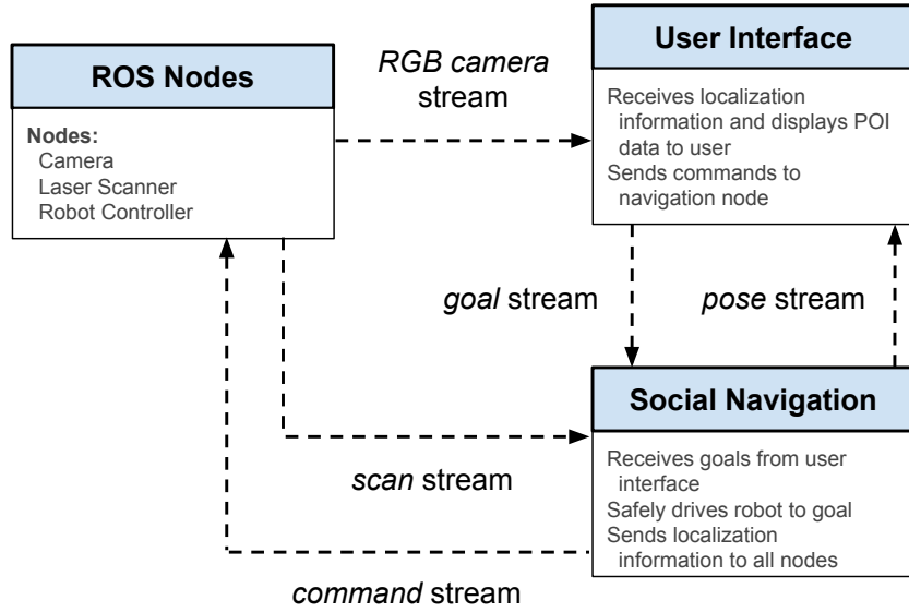
Figure IV.1: System architecture
