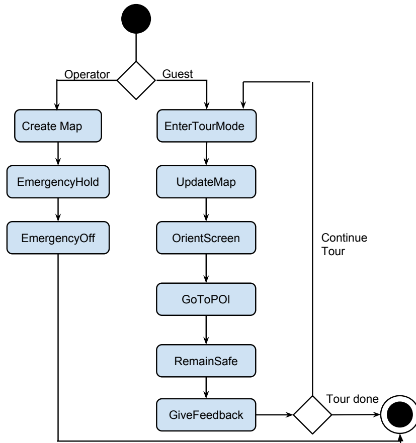
Figure IV.4: Top-level activities
